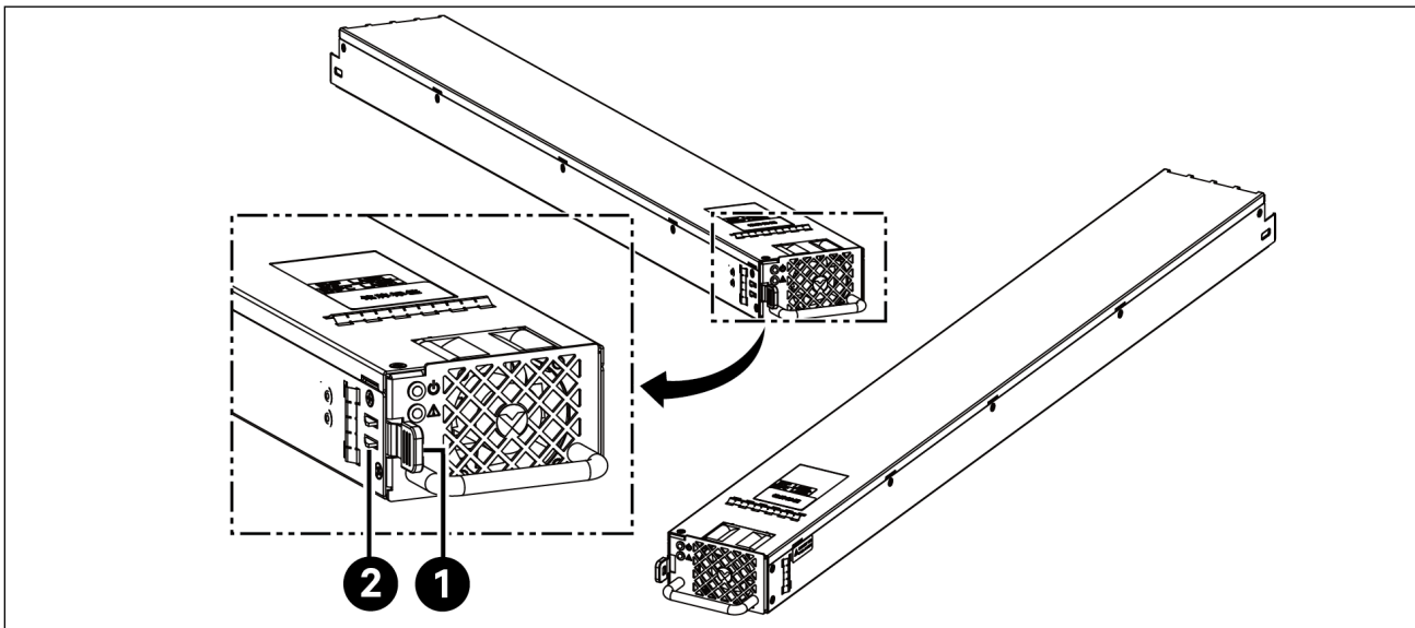
Figure 2.3 Installing Power Supply Unit
