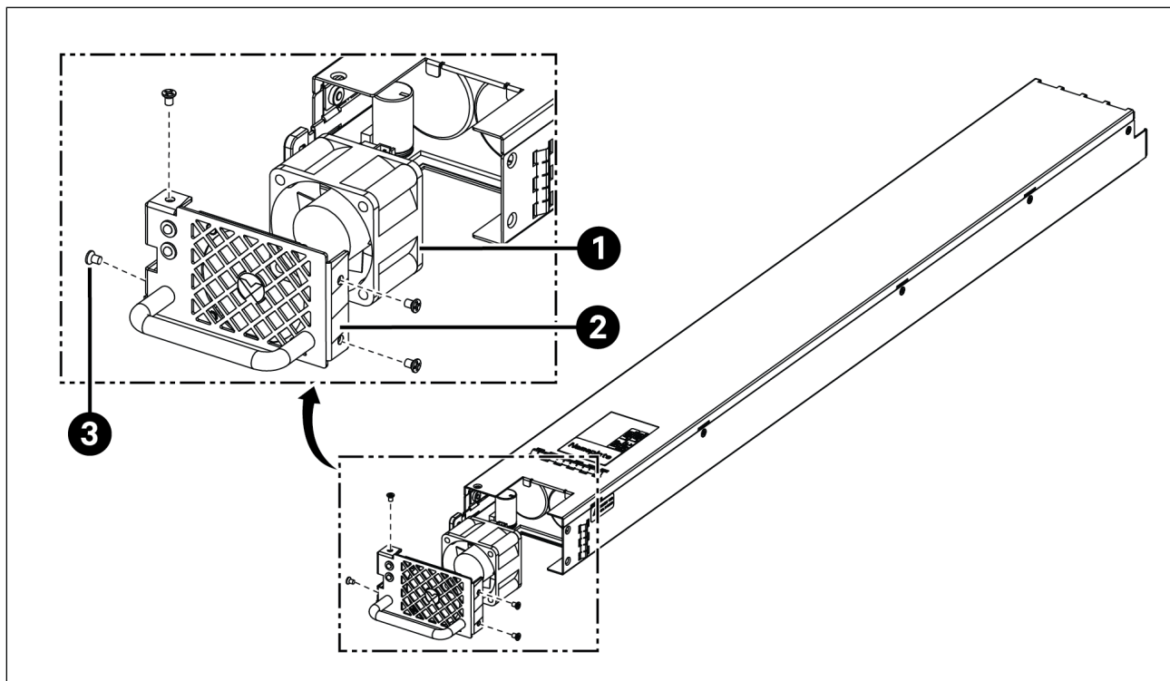
Figure 3.1 Fan Replacement
