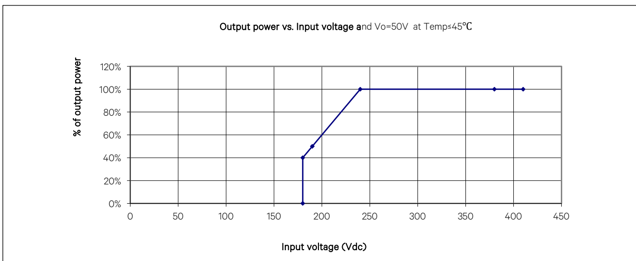
Figure 1.3 Power Based on Input Voltage at Temp \leq 45^{\circ}\text{C} and V_o = 50\text{ V} from 180 VDC to 410 VDC
