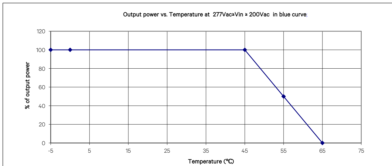
Figure 1.4 Power Derating Based on Temperature
