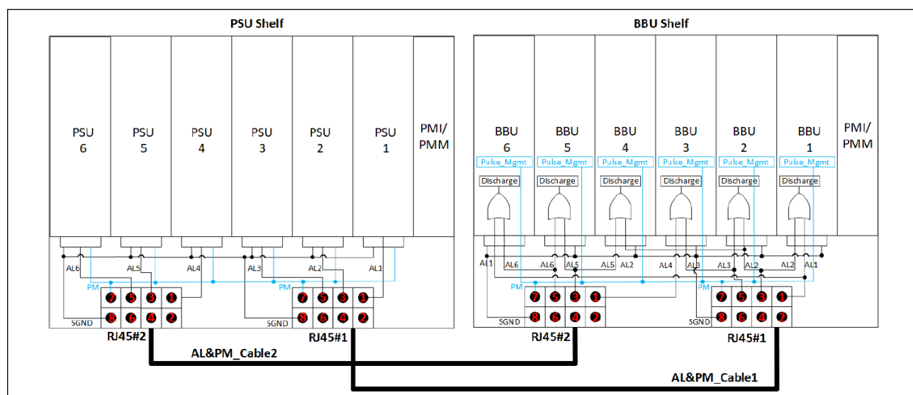
Figure 1.7 AC_Loss & Pulse Management Signals
