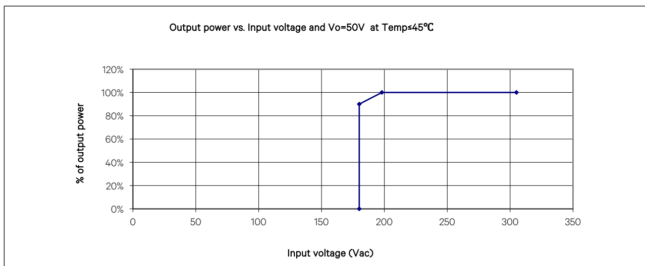
Figure 1.2 Power Based on Input Voltage at Temp \leq 45^{\circ}\text{C} and V_o = 50\text{ V} from 180 VAC to 305 VAC
