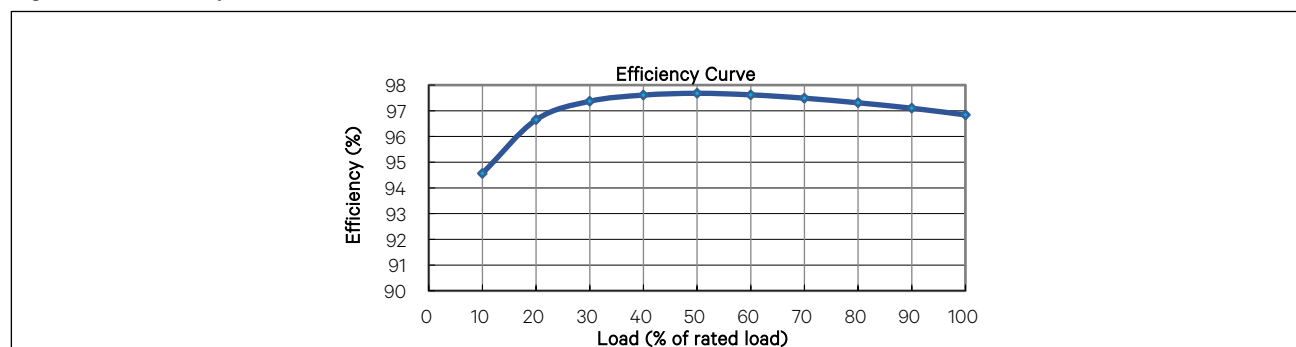
Figure 1.5 Efficiency Curve
