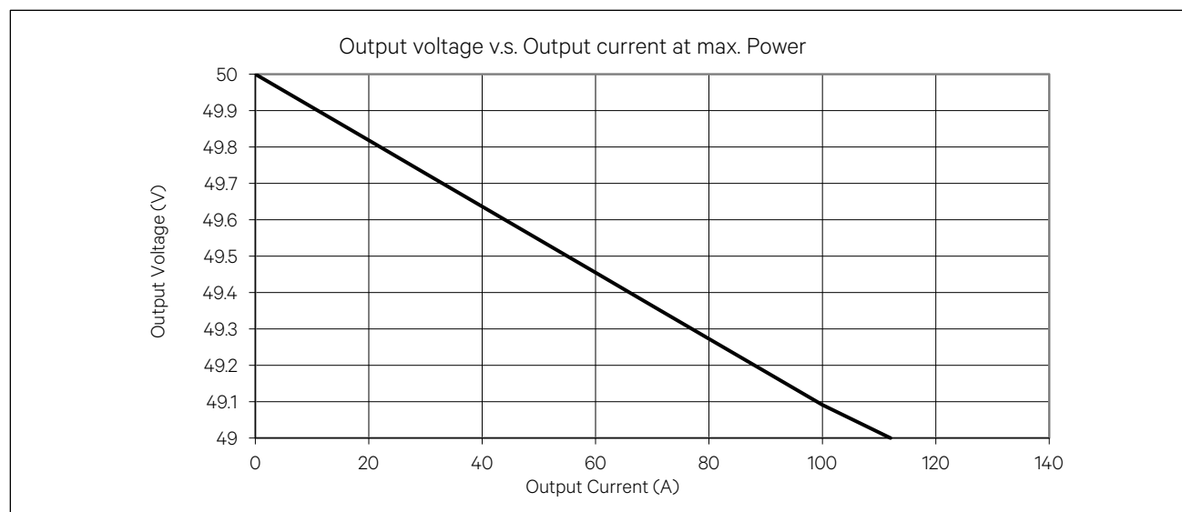
Figure 1.1 Output Voltage vs. Output Current
