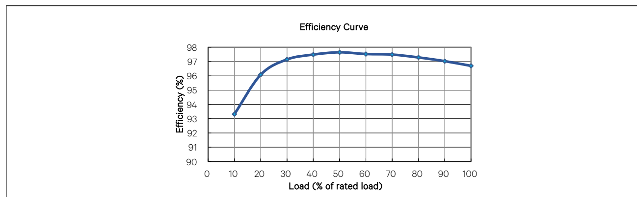
Figure 1.6 Efficiency Curve
