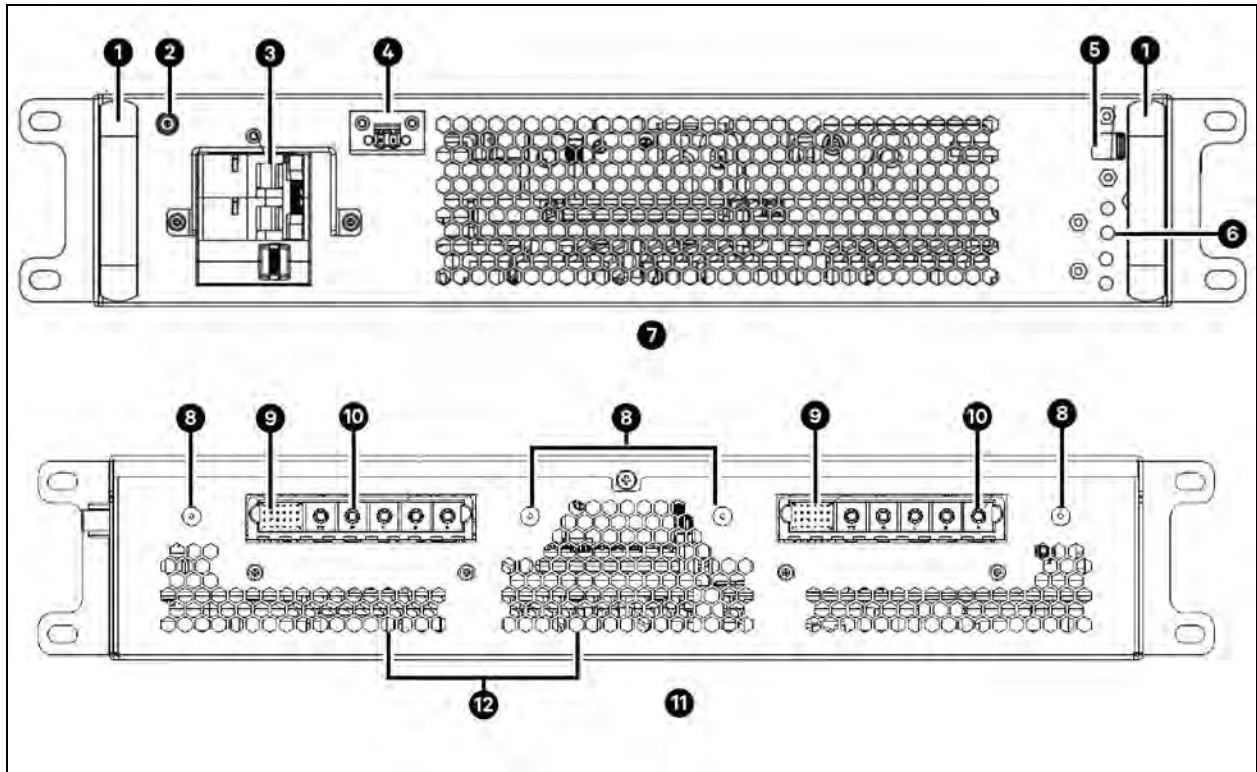
Figure 2.2 Vertiv™ Liebert® APM2 Lithium Battery Modules
