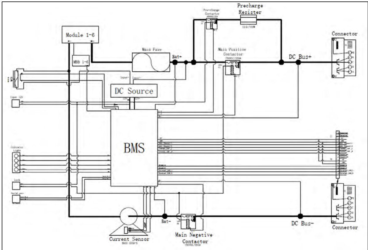
Figure 2.4 Liebert® APM2 Lithium Battery Module System Schematic Diagram
