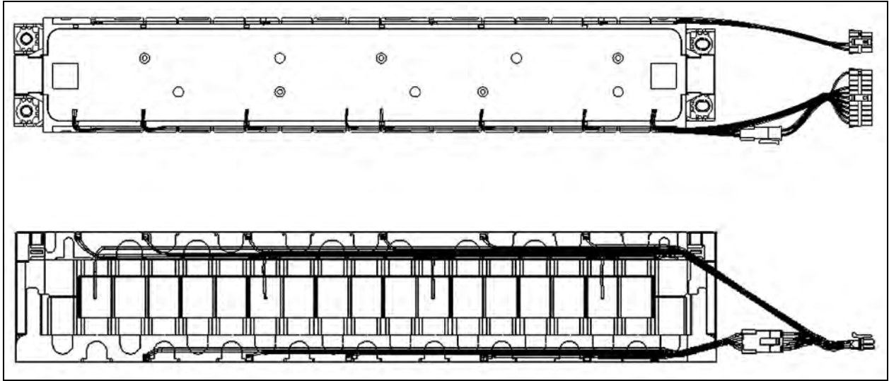
Figure 2.5 Structure Diagram of Vertiv™ Liebert® APM2 Lithium Battery Module
