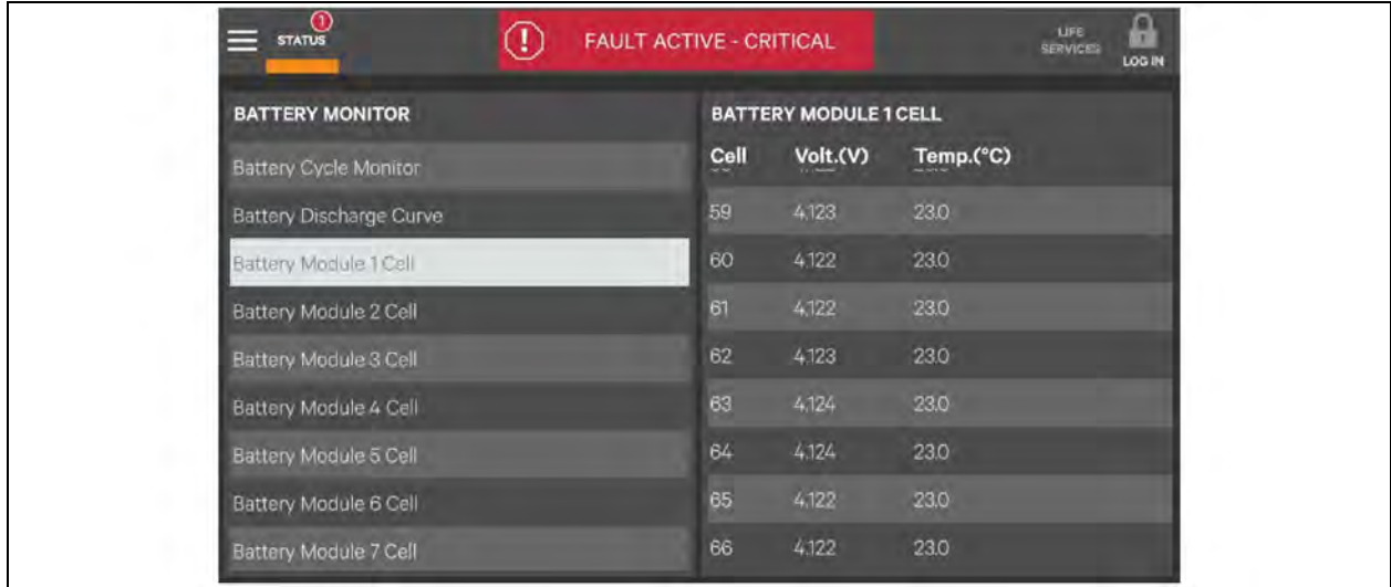
Figure 5.10 Battery Specific Voltage and Temperature Data
