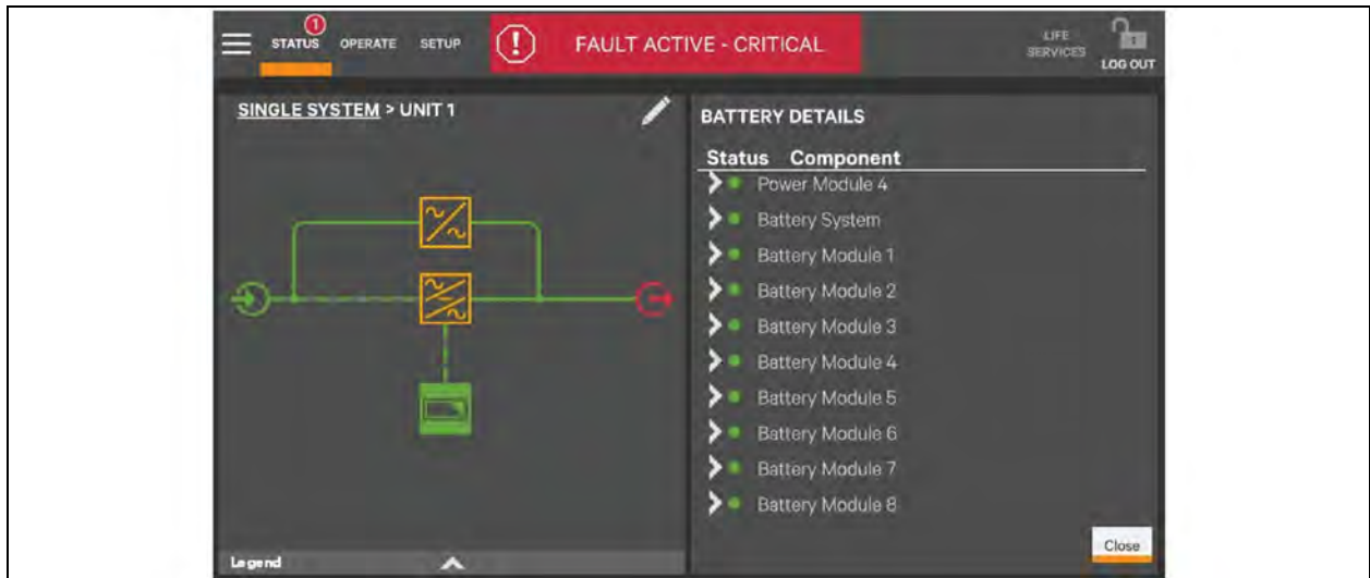
Figure 5.3 Main Screen Lithium Battery Module
