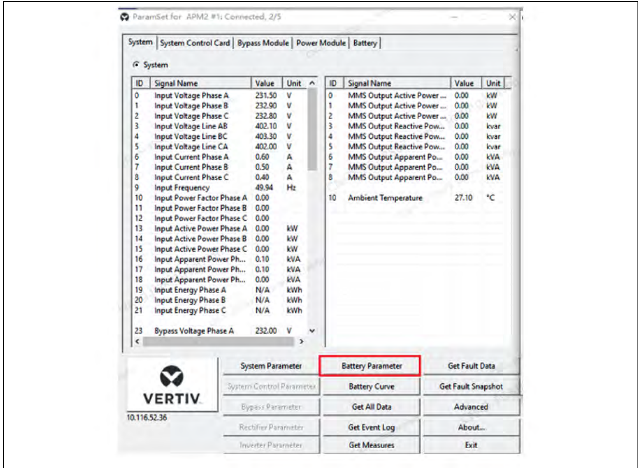
Figure 3.2 Paramset Software
