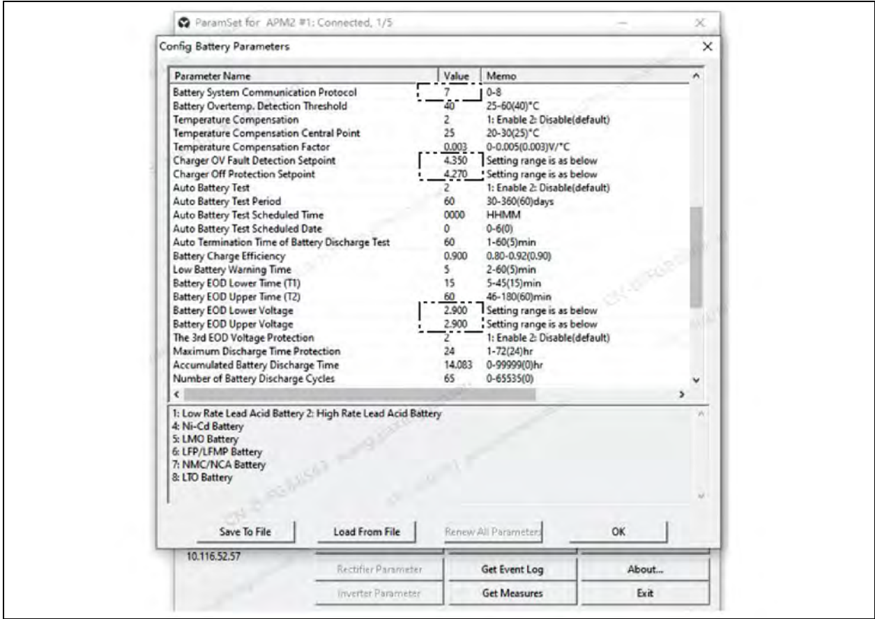
Figure 3.4 Configuration of Battery Parameters_2
